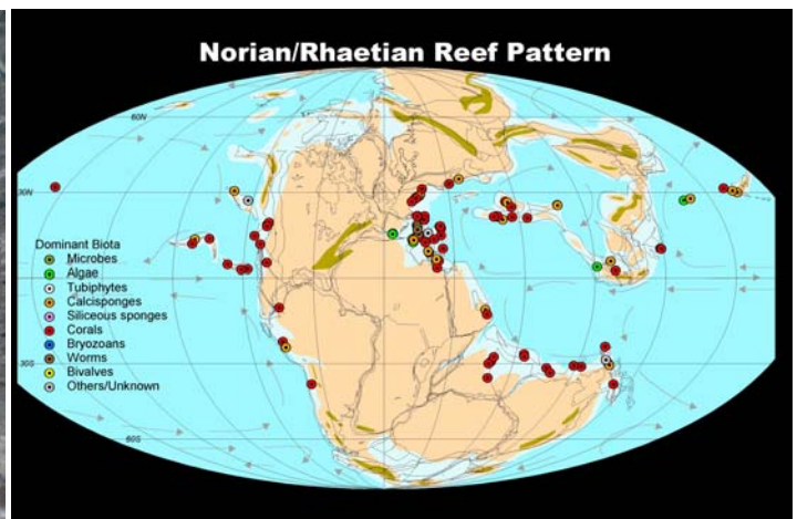
Paleogeographic reef distribution in the Norian-Rhaetian (Late Triassic)
