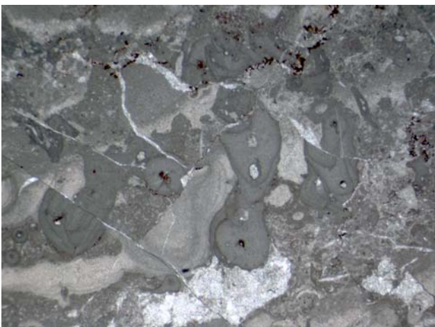
Tubiphytes reef limestone from the Permian of Texas
